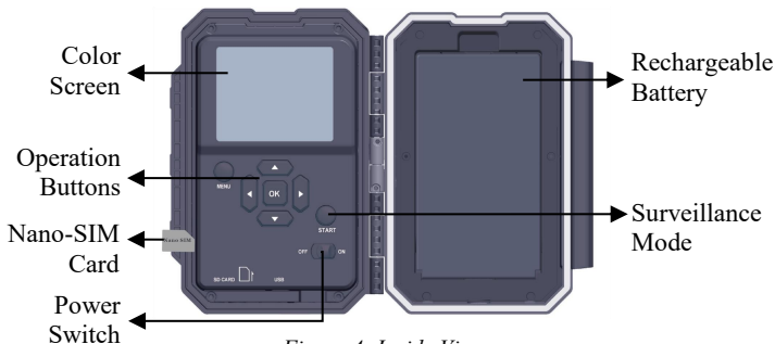
Figure 4: Inside View
