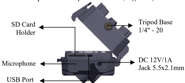
Figure 2: Bottom View
