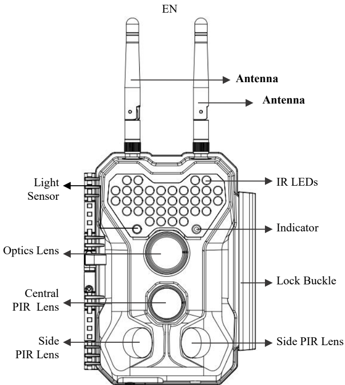
Figure 1: Front View
