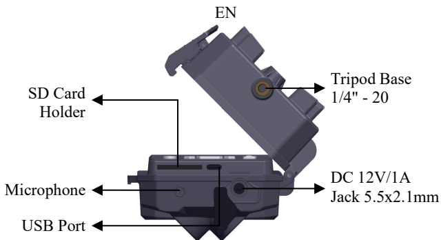
Figure 2: Bottom View
